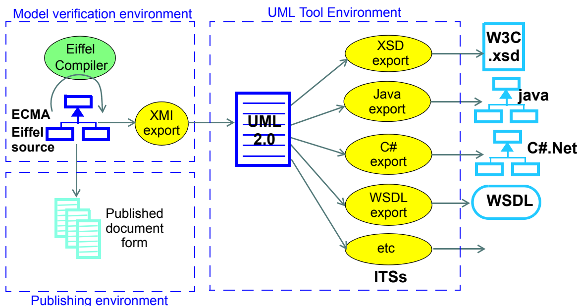
FIGURE 1 openEHR modelling environment
