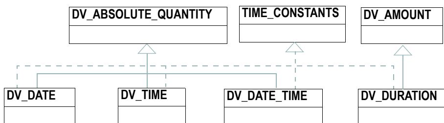
FIGURE 4 rm.data_types.quantity.date_time Package
