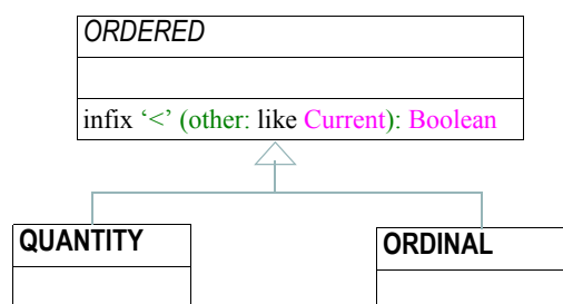
FIGURE 8 pseudo-UML for Anchored Types
